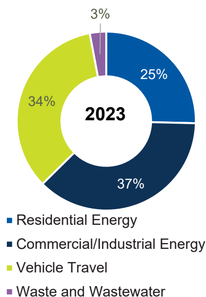
Figure 3. Hennepin County 2023 GHG Emissions by Sector
