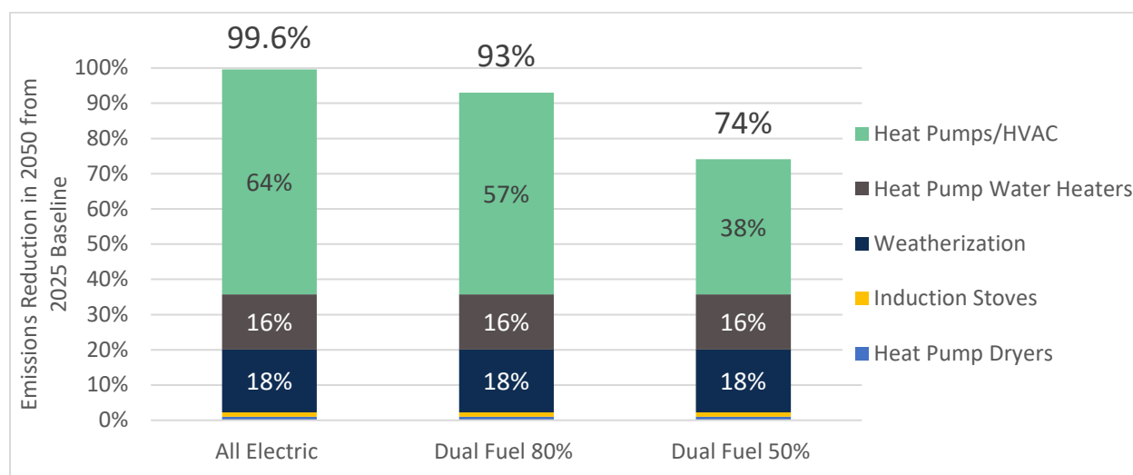
Figure 9. Emissions reductions achieved in 2050 by measure and model scenario
